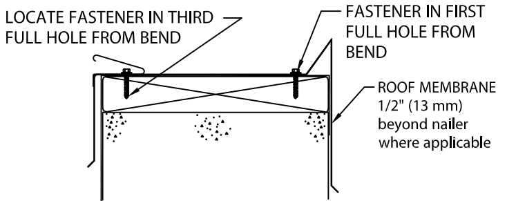
ANCHOR CLIP FASTENING-DETAIL A
